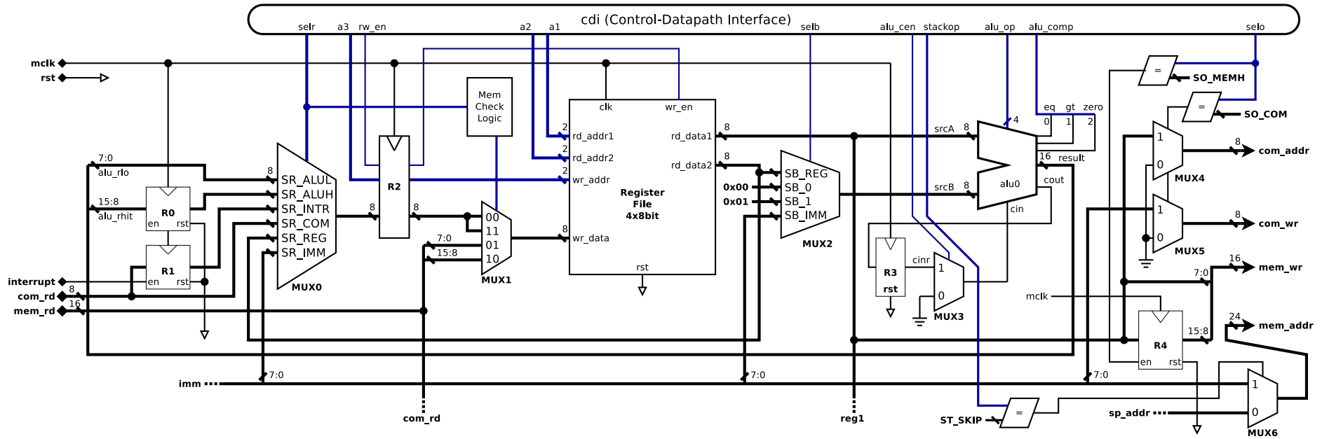
Figure 3.3.4: Digital diagram of RISC8 datapath
