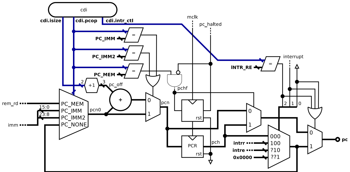
Figure 3.3.1: Digital diagram of RISC program counter
