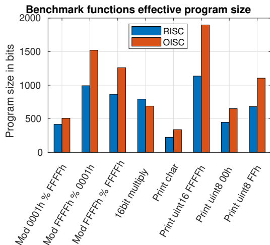
Figure 5.2.2: Bar graph showing effective size in bits each benchmark function is taking in program memory.
