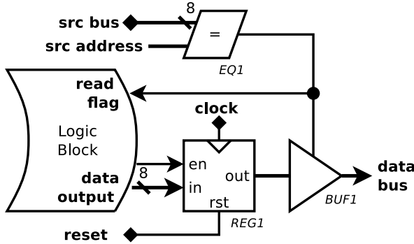
Figure 4.2.3: OISC processor data bus to source connection logic
