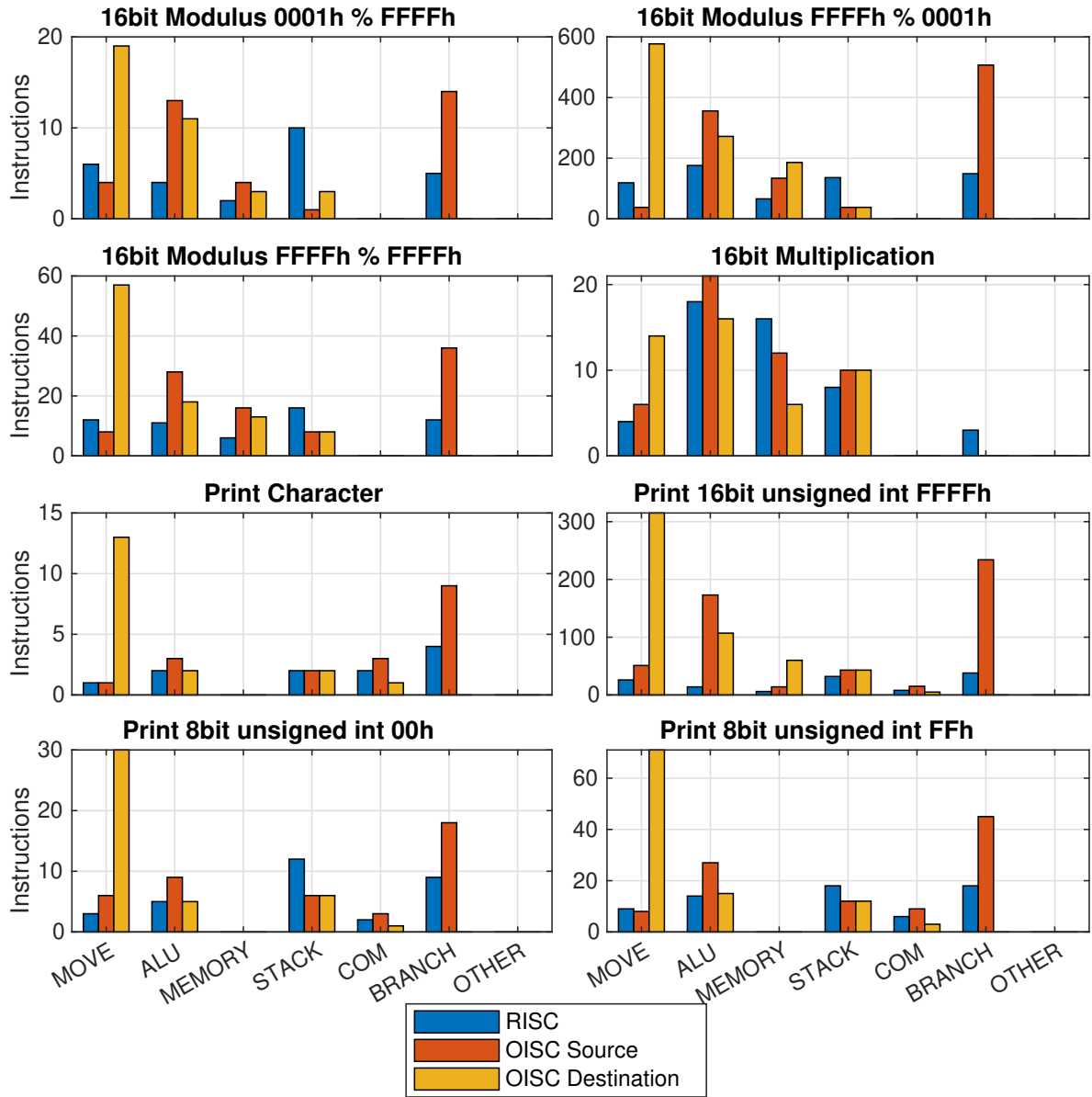
Figure 5.2.1: Graph of instruction composition for every benchmark program.
